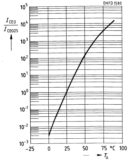
Dunkelstrom I_{CEO}/I_{CEO25} = f(T_A) V_{CE} = 25 \text{ V}, E = 0
