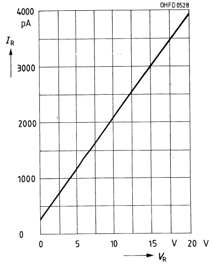
Dunkelstrom I_R = f(V_R) E = 0
