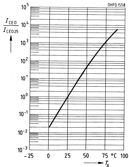
Dunkelstrom I_{CEO}/I_{CEO25} = f(T_A) V_{CE} = 25 V, E = 0
