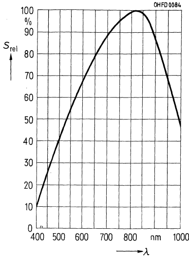
Relative spektrale Empfindlichkeit S_{rel} = f(\lambda) BPX 90
