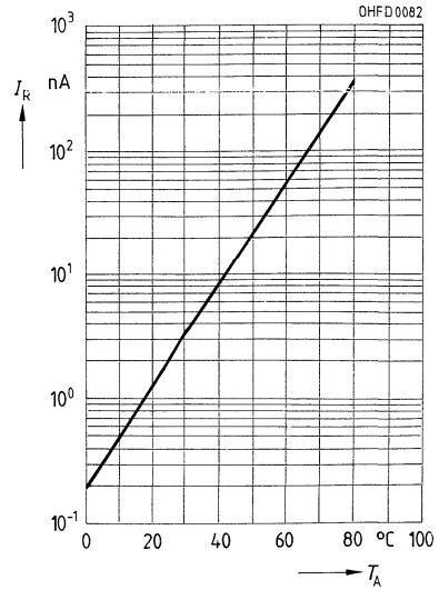
Dunkelstrom I_R = f(T_A) V_R = 10 \text{ V}, E = 0
