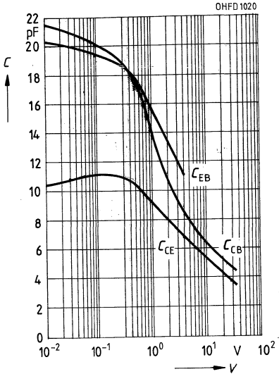
Kapazität C = f(V) f = 1 \text{ MHz}, E = 0
