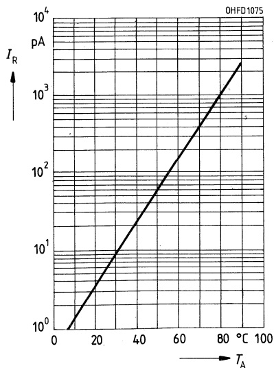
Dunkelstrom I_R = f(T_A) V_R = 1 \text{ V}, E_v = 0
