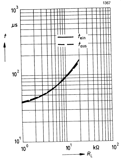
Schaltzeiten, t = f(R_L) T_A = 25^\circ\text{C, } I_C = 100 \mu\text{A, } I_F = 10 \text{ mA}
