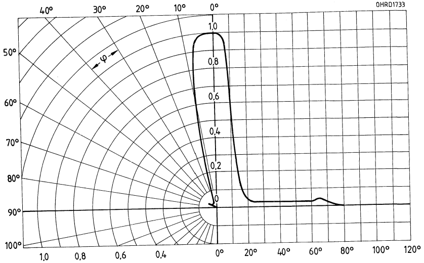
Abstrahlcharakteristik I_{rel} = f(\lambda) SFH 414
