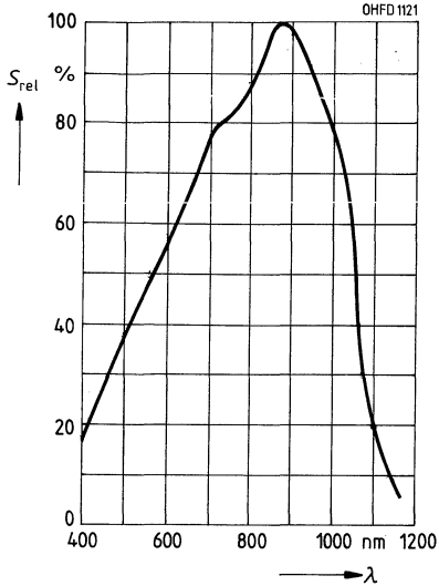
Relative spektrale Empfindlichkeit S_{rel} = f(\lambda) SFH 320
