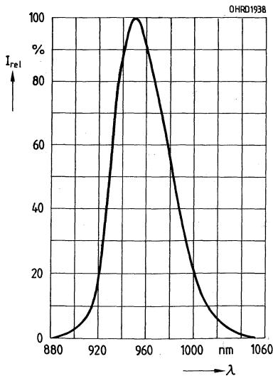
Relative spektrale Emission
