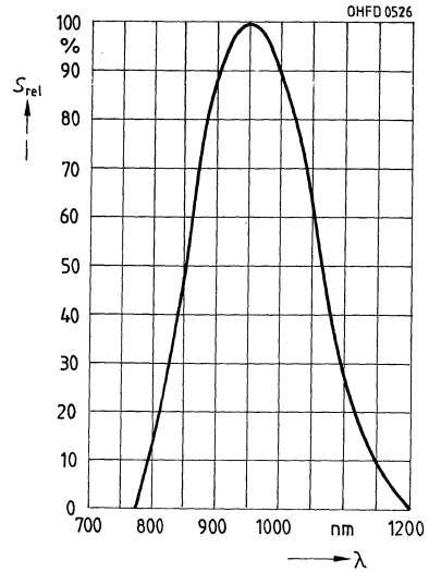
Relative spektrale Empfindlichkeit S_{rel} = f(\lambda) BPX 90 F
