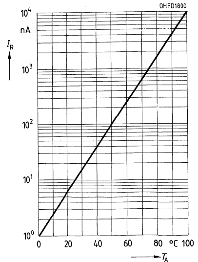
Dunkelstrom I_R = f(T_A) V_R = 20 \text{ V}, E = 0
