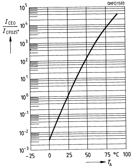
Dunkelstrom I_{CE0}/I_{CE0\ 25} = f(T_A) , V_{CE} = 25\text{ V}, E = 0
