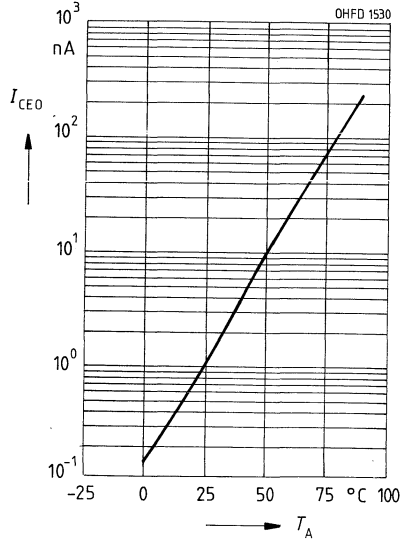
Dunkelstrom I_{CE0} = f(T_A) V_{CE} = 25 \text{ V}, E = 0
