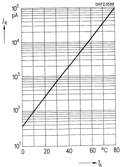
Dunkelstrom I_R = f(T_A) V_R = 7 \text{ V}, E = 0
