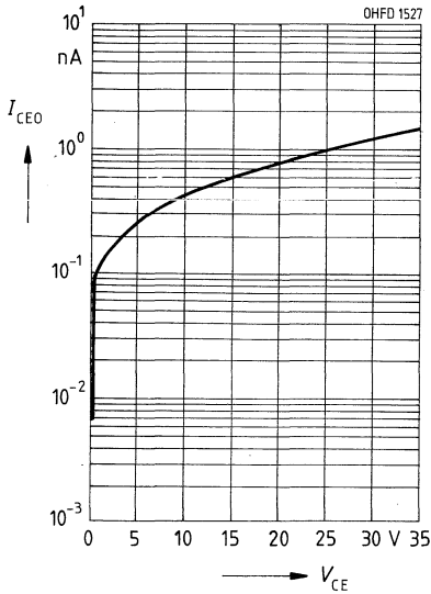
Dunkelstrom I_{CE0} = f(V_{CE}) E = 0
