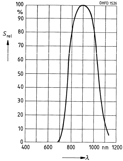
Relative spektrale Empfindlichkeit S_{rel} = f(\lambda) SFH 320 F
