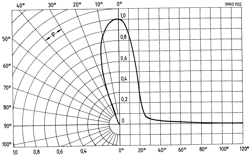
Abstrahlcharakteristik I_{rel} = f(\varphi) SFH 475
