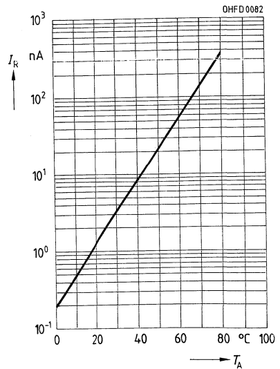
Dunkelstrom I_R = f(T_A) V_R = 10, E = 0
