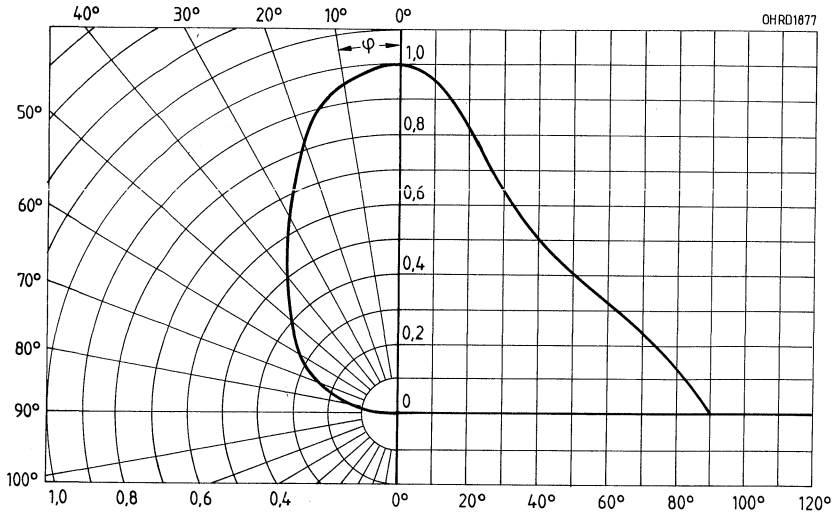
Abstrahlcharakteristik I_{rel} = f(\varphi)
