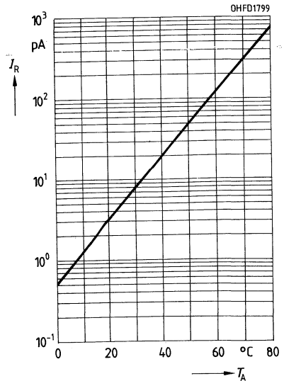
Dunkelstrom I_R = f(T_A) V_R = 1 \text{ V}, E = 0
