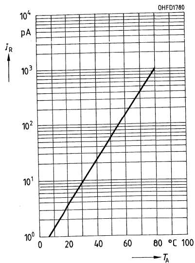
Dunkelstrom I_R = f(T_A) E_V = 0, V_R = 1 \text{ V}
