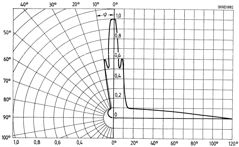
Abstrahlcharakteristik I_{rel} = f(\varphi) LD 274
