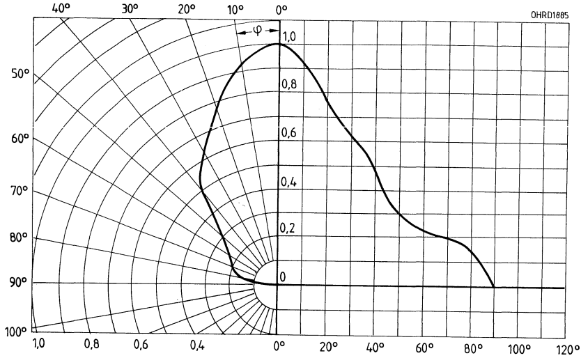
Abstrahlcharakteristik I_{rel} = f(\varphi) SFH 402
