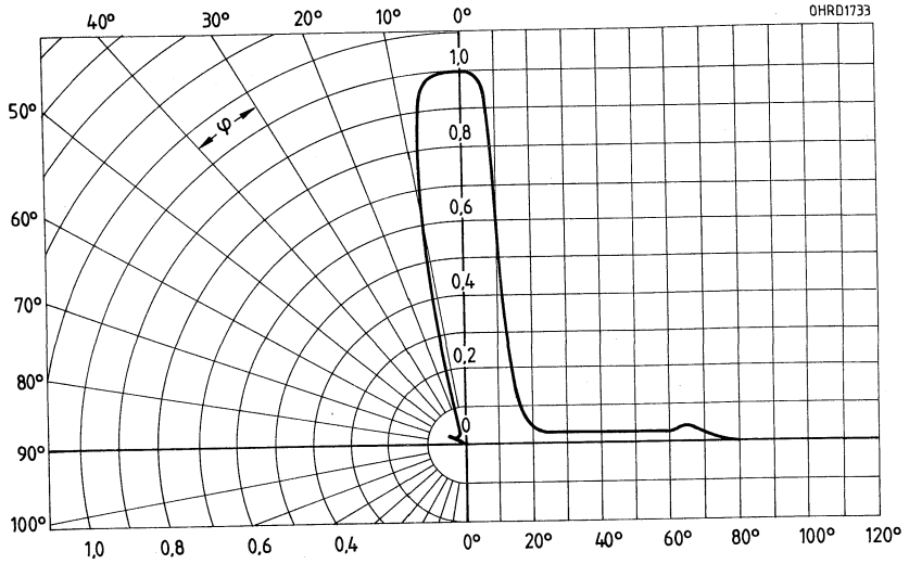
Abstrahlcharakteristik I_{rel} = f(\varphi) SFH 474
