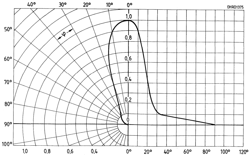
Abstrahlcharakteristik I_{rel} = f(\varphi) LD 275
