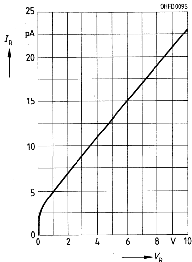
Dunkelstrom I_R = f(V_R) E_v = 0
