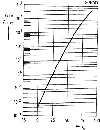
Dunkelstrom I_{CE0}/I_{CE025} = f(T_A) V_{CE} = 25 \text{ V}, E = 0
